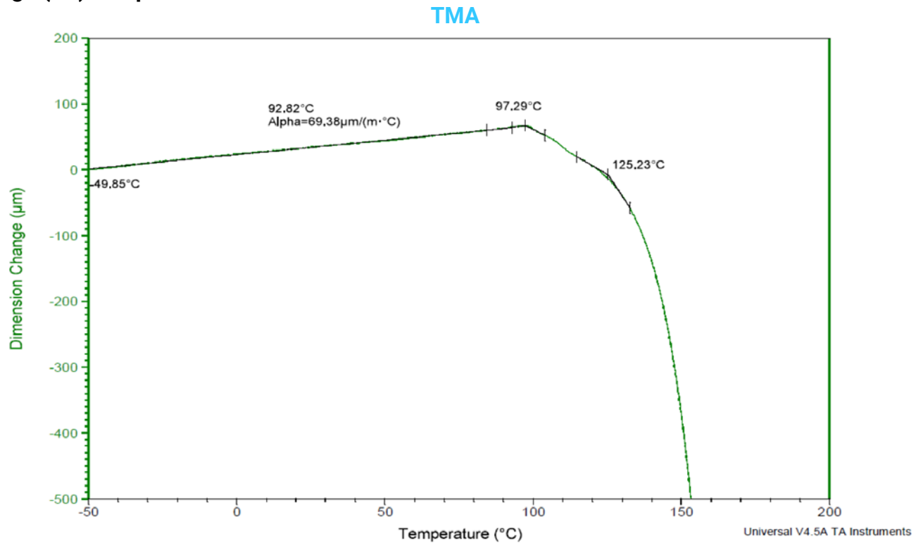
Figure 3: Dimension change data as a function of temperature for the ABS-M30 Black On Edge (XZ) sample.
