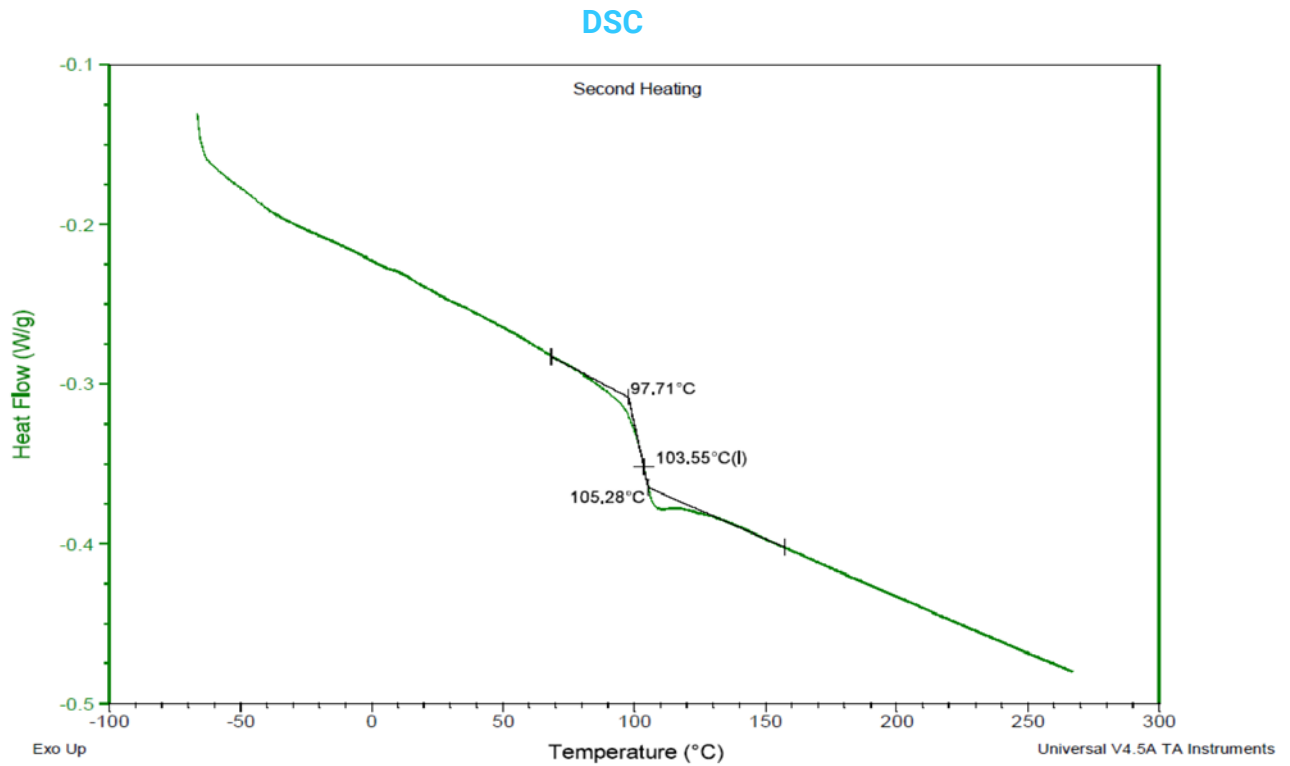
Figure 1: 2nd heating scan DSC data for the ABS-M30 Black Flat (XY) sample.
